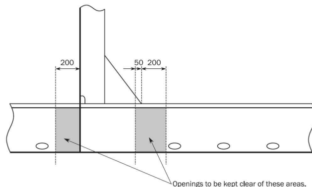
Figure 12 : Location of air and drain holes
