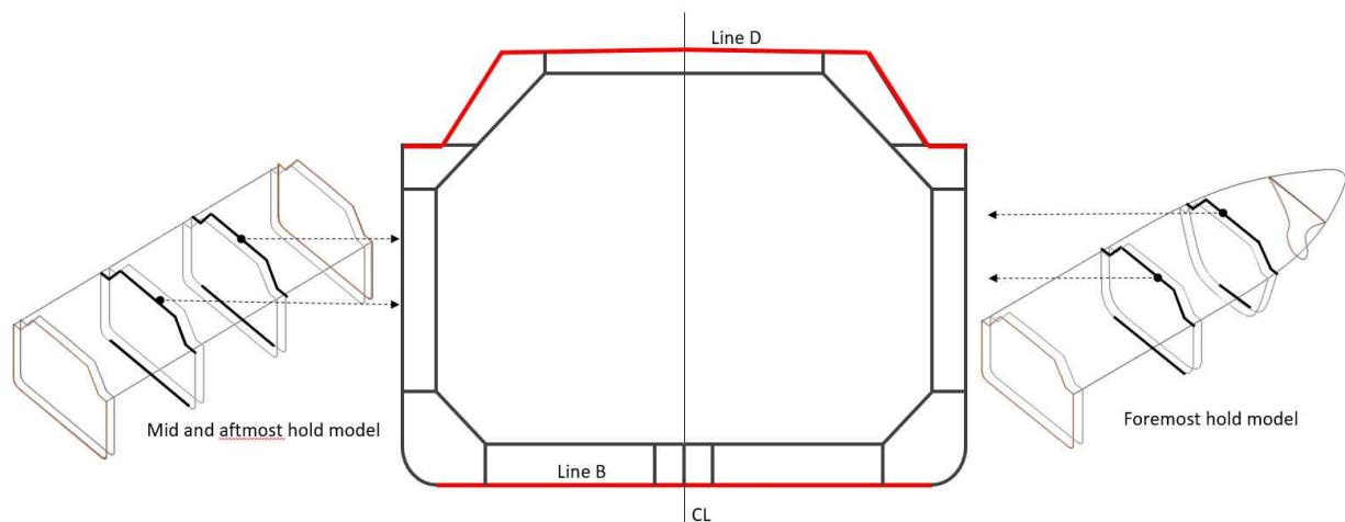
Figure 9 : Additional LM3-I Boundary conditions applied at the model
