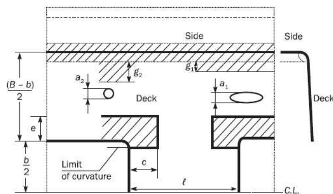
Figure 14 : Position of openings in strength deck
