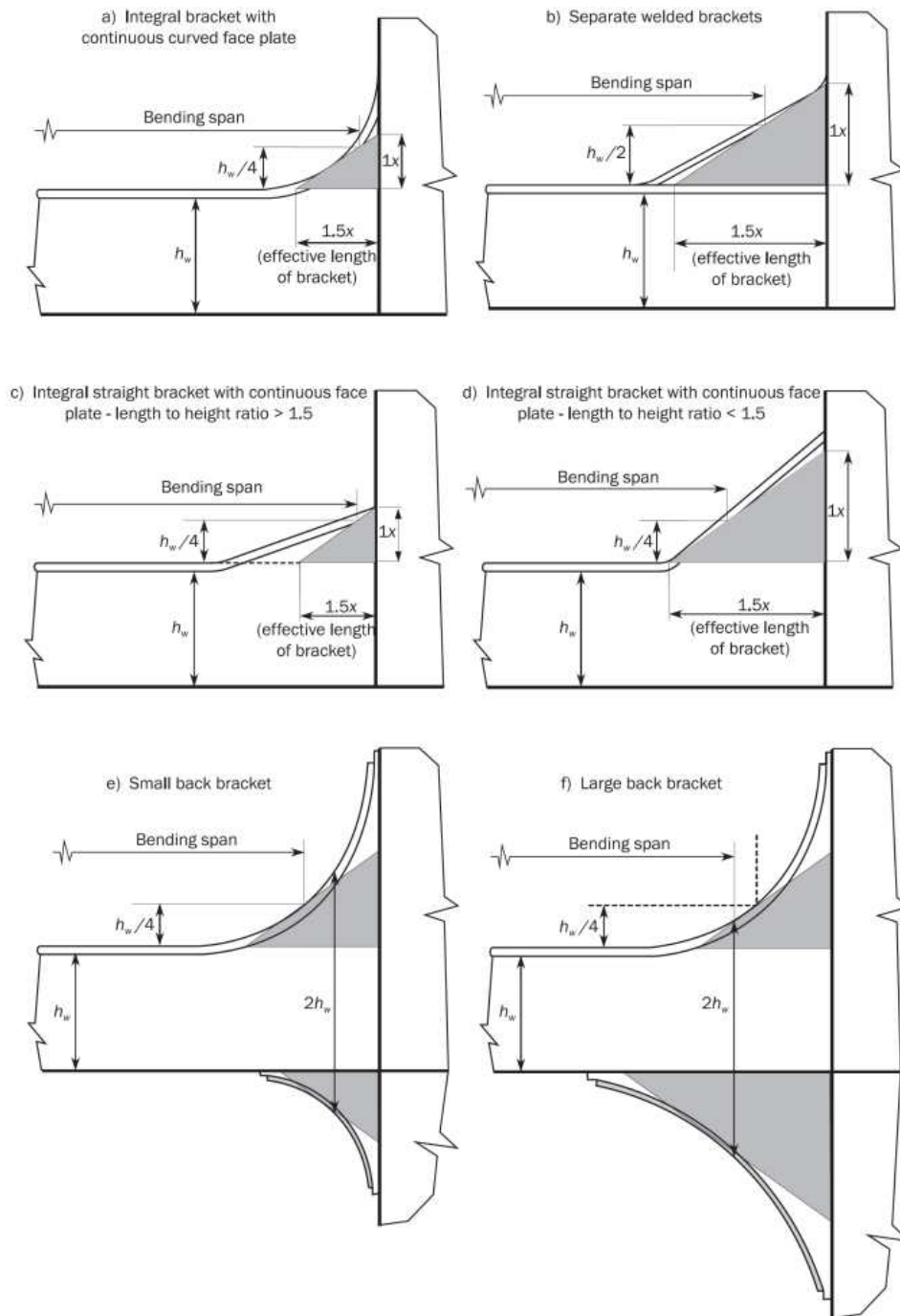
Figure 7 : Effective bending span of primary supporting member
