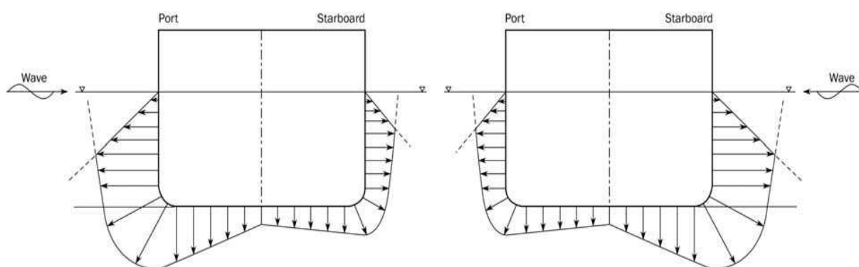
Figure 7 : Transverse distribution of dynamic pressure for BSP-2P(left)와 BSP-2S(right) load cases
