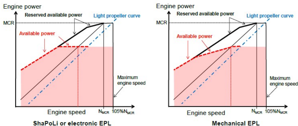
Figure 1: Engine load diagram on Shaft/Engine Power Limitation
