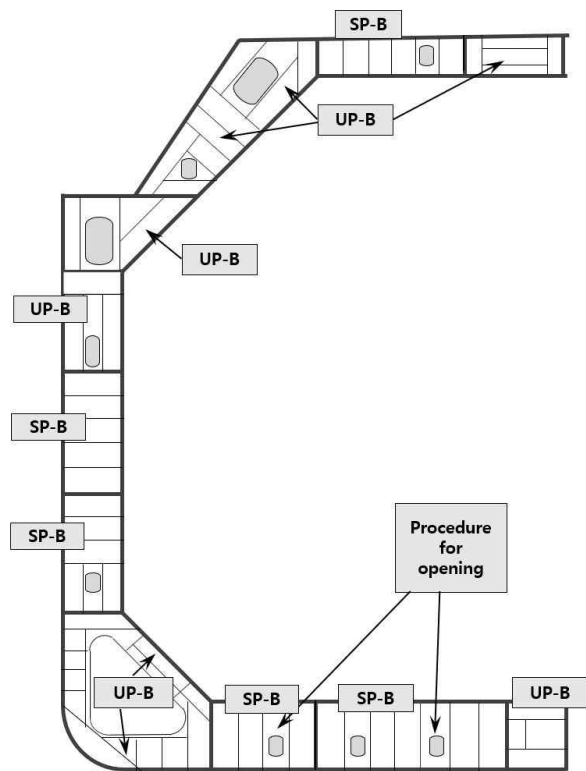
Figure 2 : Transverse web frames for liquid natural gas carrier (Partly shown) (2023)
