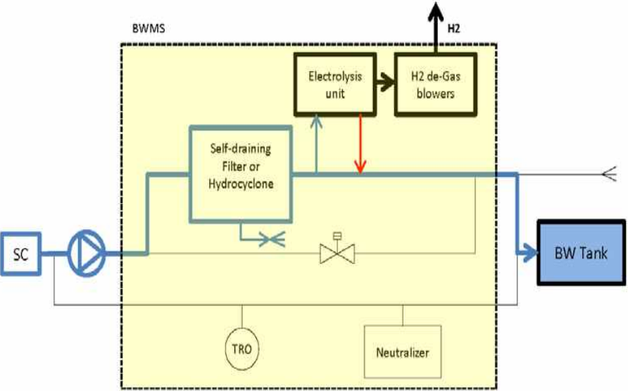
Ballasting operation:
