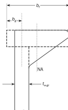
Figure 4 : Bulb profile and equivalent built-up profile
