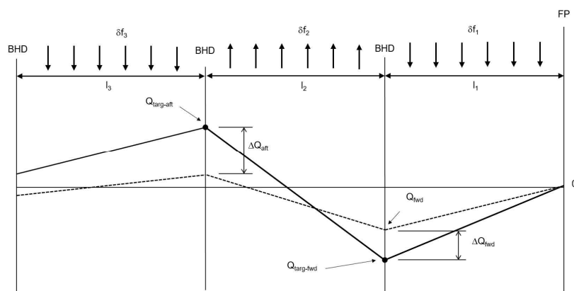
Figure 12 : Shear force adjustment at two bulkheads (aft BHD Q_{targ-afd} (+ve) , fore BHD Q_{targ-fwd} (-ve) )
