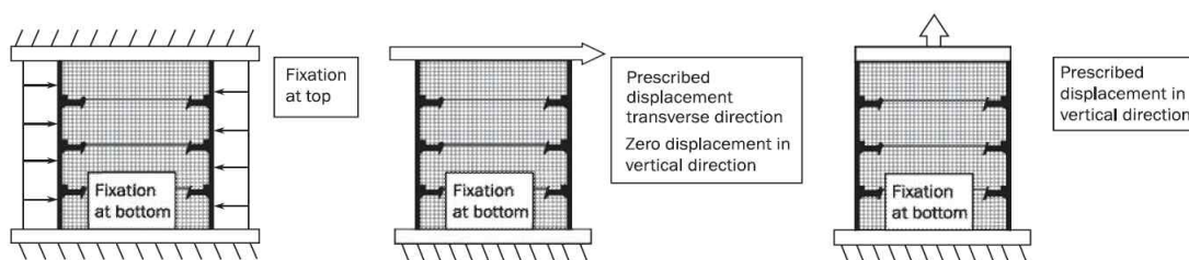
Figure 3 : Load application and boundary conditions – FE model for verification of alternative design
