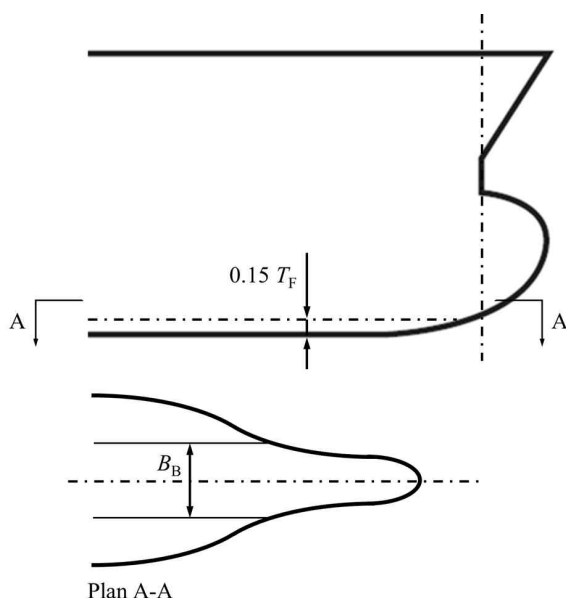
Figure 2 : Breadth of bottom at the height 0.15 T_F
