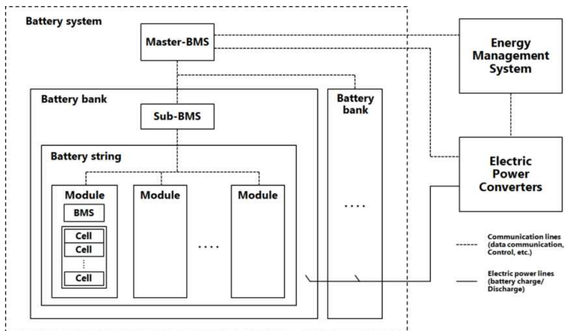
Fig 1 Block diagram of battery system (2019)
