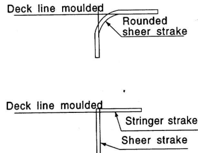
Fig 3.3.3 Deck Corners
