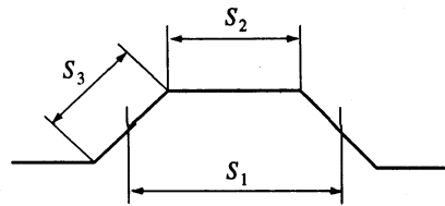
Fig 3.3.1 Corrugated Bulkheads
