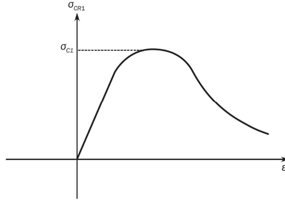
Figure 7 : Load-end shortening curve \sigma_{CR1} - \varepsilon for beam column buckling
