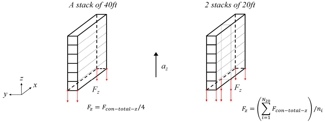
Figure 3 : Vertical container load component in hold
