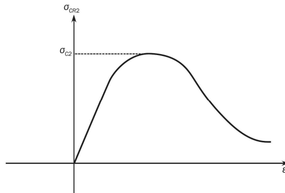
Figure 8 : Load-end shortening curve \sigma_{CR2} - \varepsilon for flexural-torsional buckling
