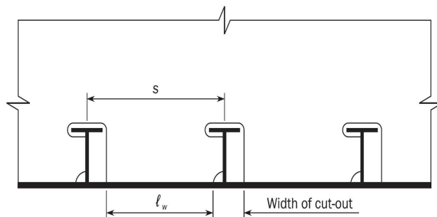
Figure 6 : Effective material in web cut-outs for stiffeners
