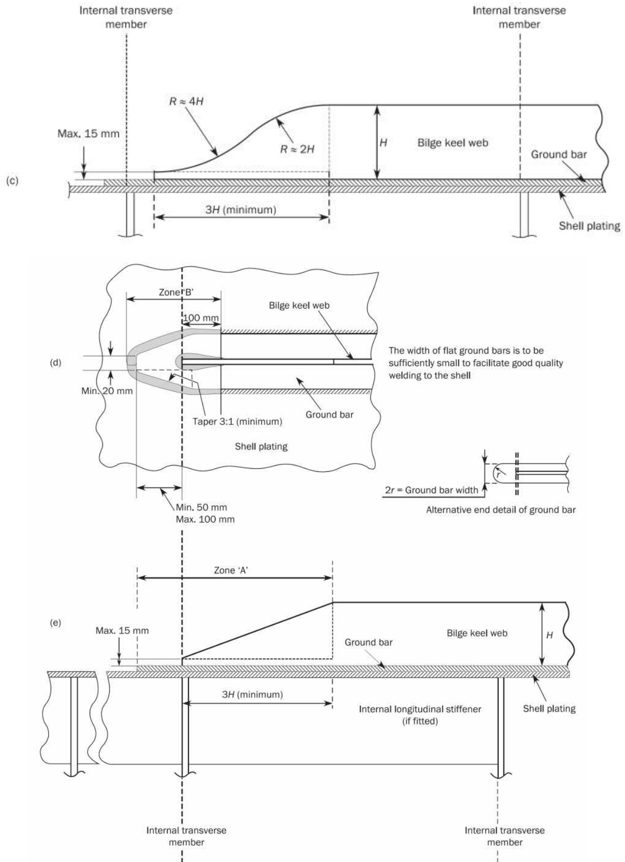
Figure 19 : Bilge keel end design (continued)
