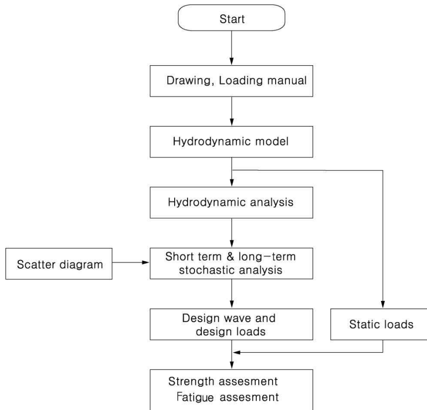
Figure 1 Flow chart of direct wave load analysis
