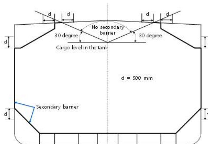
Figure 3.3 Application range extension of secondary steel for Type A tank
