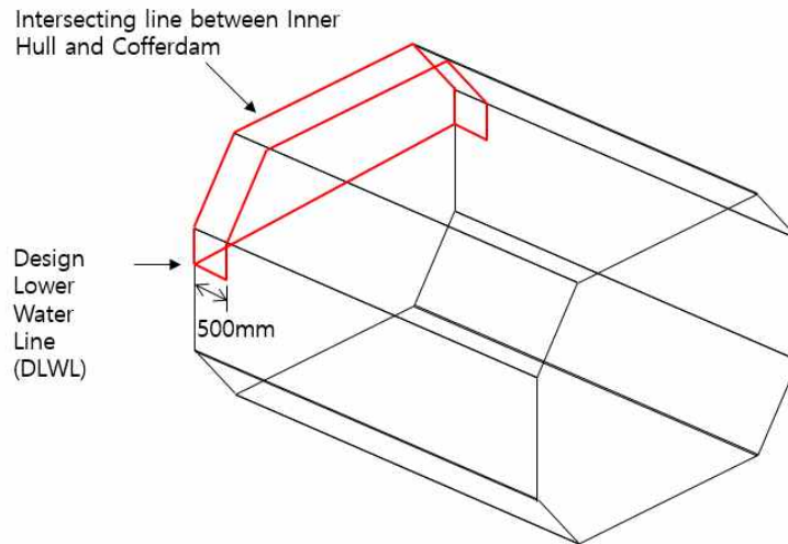
Figure 2.11 Important consideration range in steel selection
