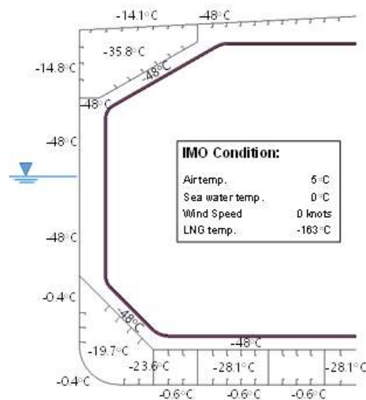
Figure 3.1 Temperature calculation for Type A tank using analytical method
