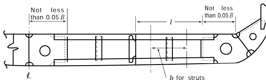
Fig 10.7.1 Open Floors
