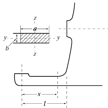
Fig 10.2.1 Shoe piece
