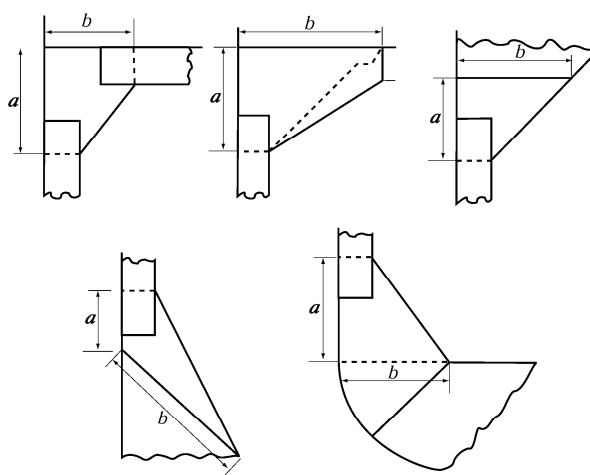
Fig 10.1.1 Measurement of a and b for arms
