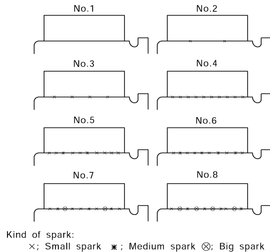
Fig 6.1.5 spark on surface of commutator
