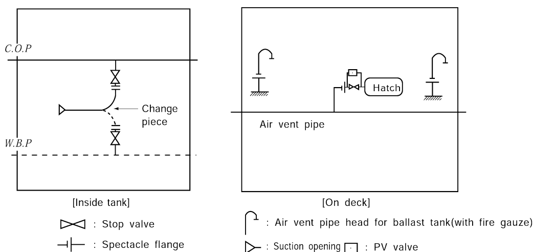
Fig 7.1.31 Example of piping arrangement for a tank used as cargo oil tank and ballast tank in alternative use
