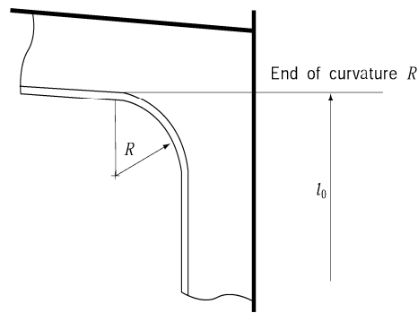
Fig 7.2.13 Measurement of l
