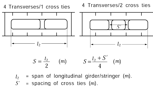
Fig 7.1.25 Value of S
