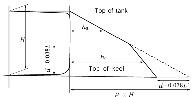
Fig 7.1.1. Measurement of h_0
