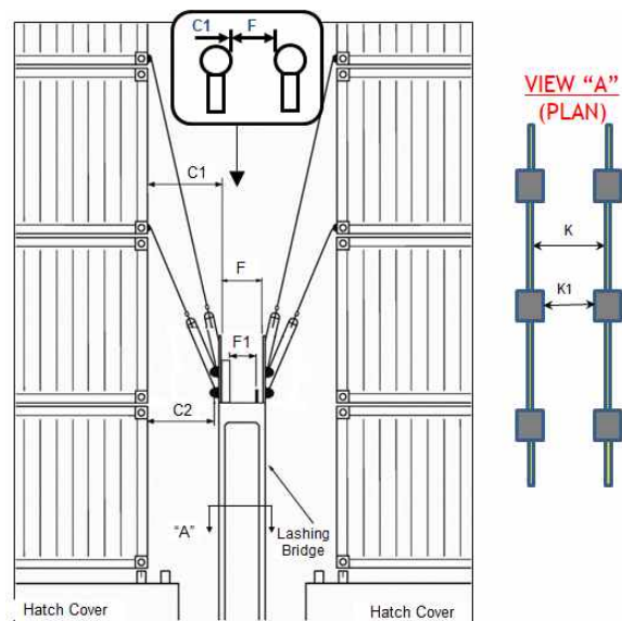
Fig 2 Lashing bridge
