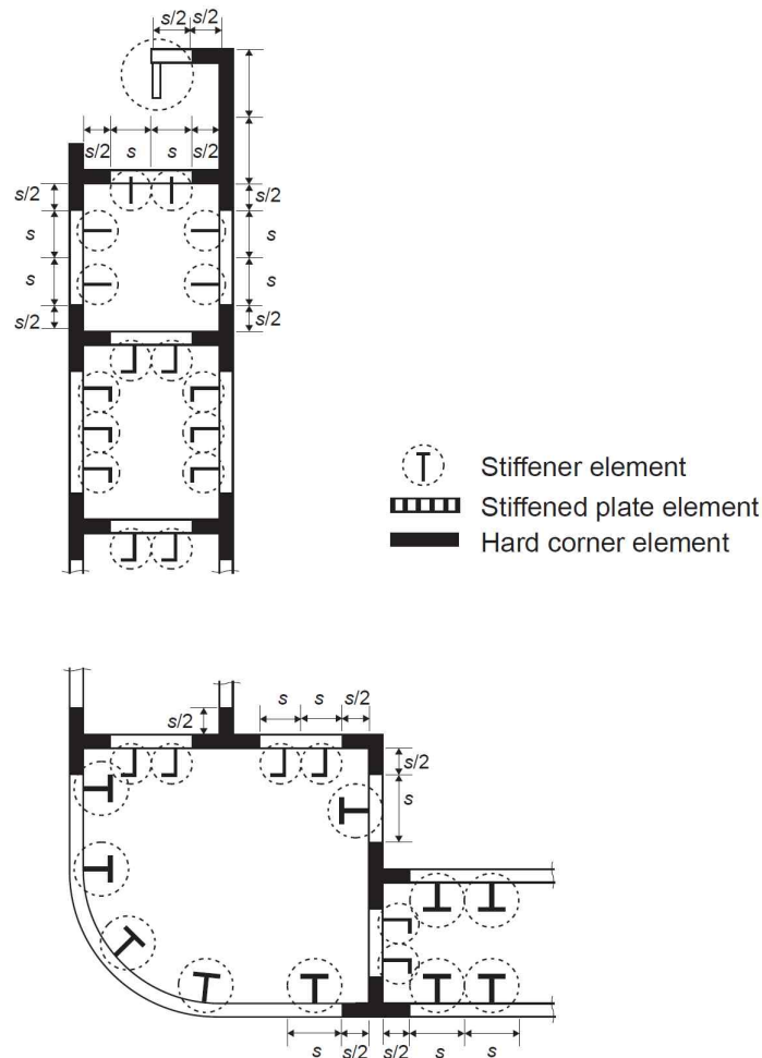
Fig A3.3 Examples of the configuration of stiffened plate elements, stiffener elements and hard corner elements on a hull section
