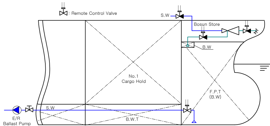
Fig 6 Application example
