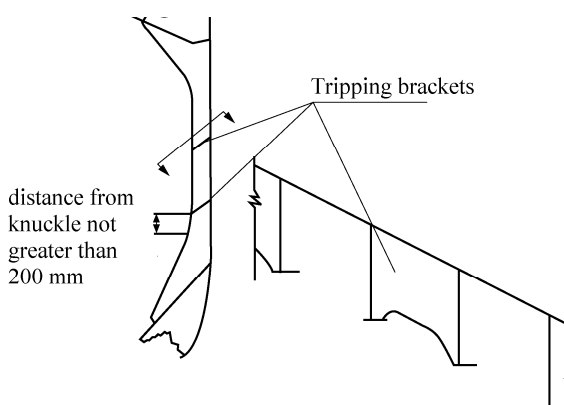
Fig 7.3.25 Tripping brackets
