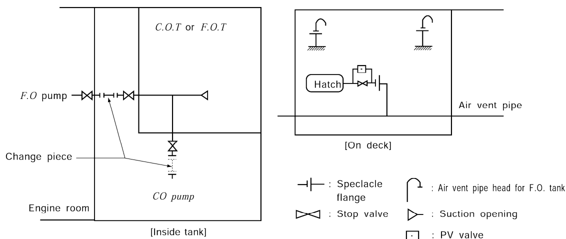
Fig 7.1.32 Example of piping arrangement for a tank used as cargo oil tank and fuel oil tank in alternative use
