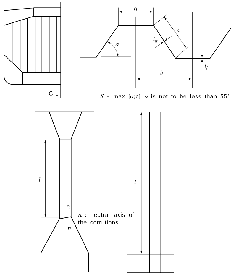
Fig 7.3.16 Measurement of S and l
