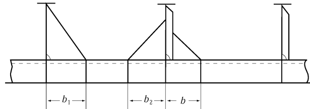
Fig. 7.1.8 Measurement of b , b_1 and b_2
