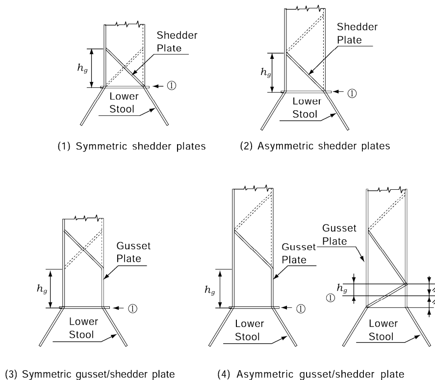
Fig 4 Shedder plates and Gusset plates
