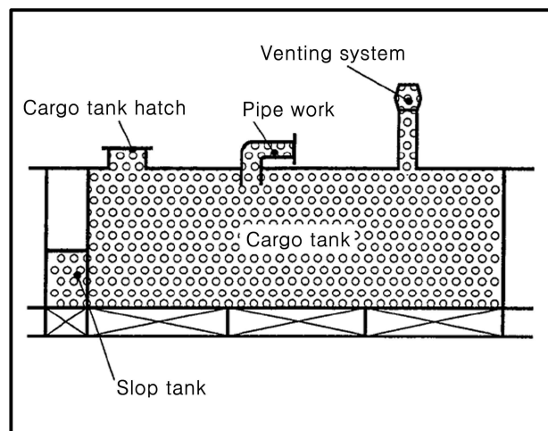
Fig 7.1.34 Example of (1) (A) zone 0
