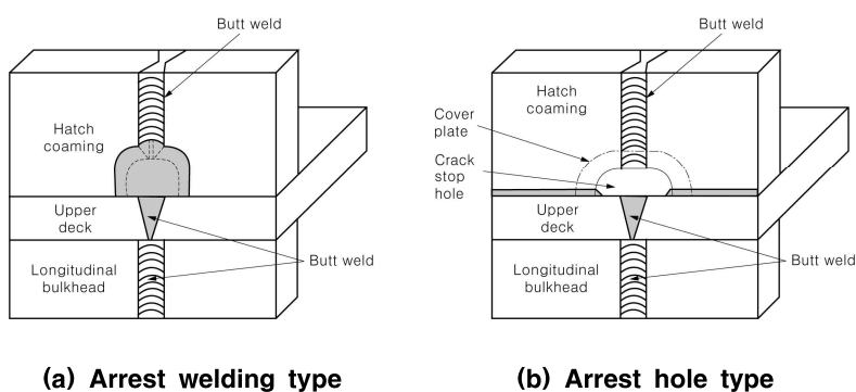
Fig 6 An example of joint arrangement for arresting the brittle crack propagation
