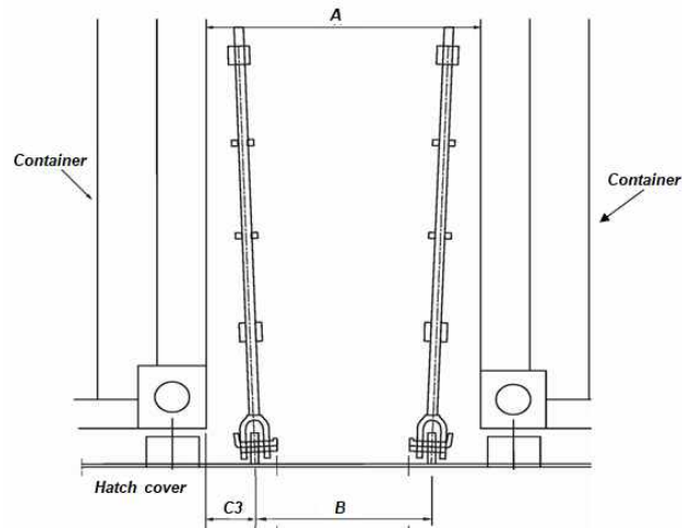
Fig 1 Work area between container stacks
