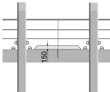
Fig 5 Toe boards
