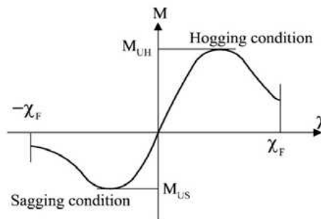
Fig 7.4.11 Bending moment M versus curvature \chi
