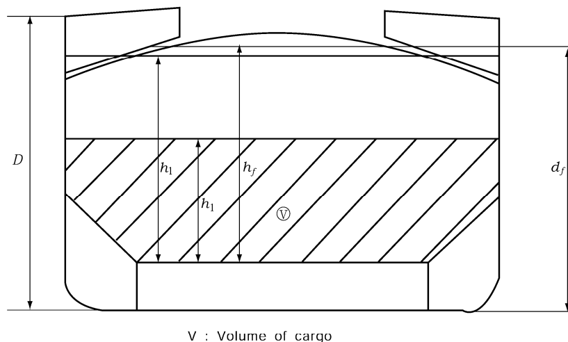
Fig. 7.3.12 Measurement of d_f , d_f , h_1 and h_f
