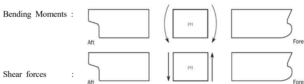
Fig 7.4.4 Sign conventions of bending moments and shear forces
