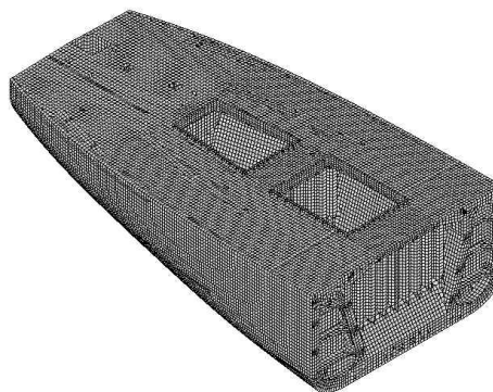
Fig 5 Example of Aft model
