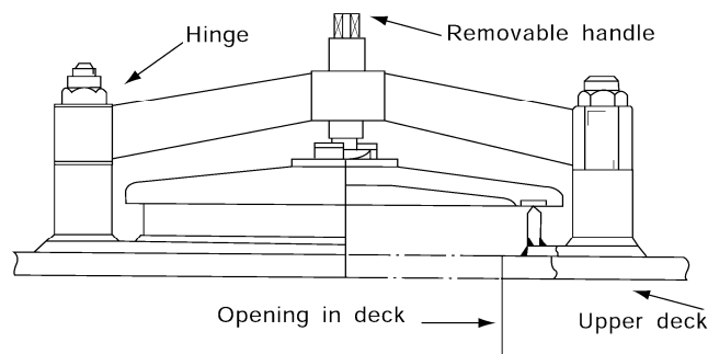
Fig 7.1.9 Cover of tank cleaning hatch
