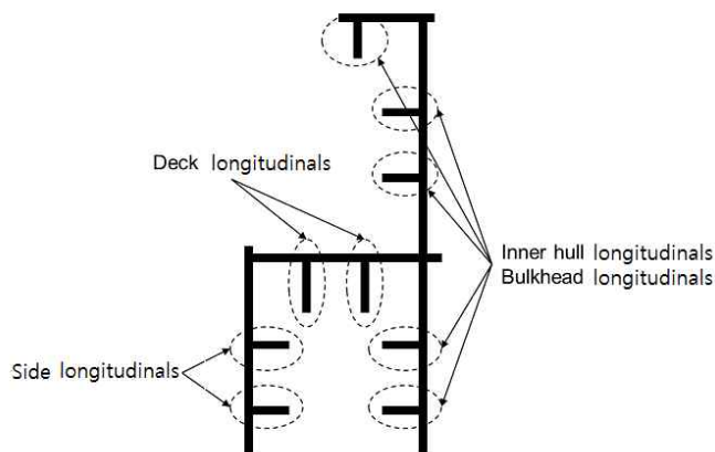
Fig 1 Upper Flange Longitudinal Structural Members
