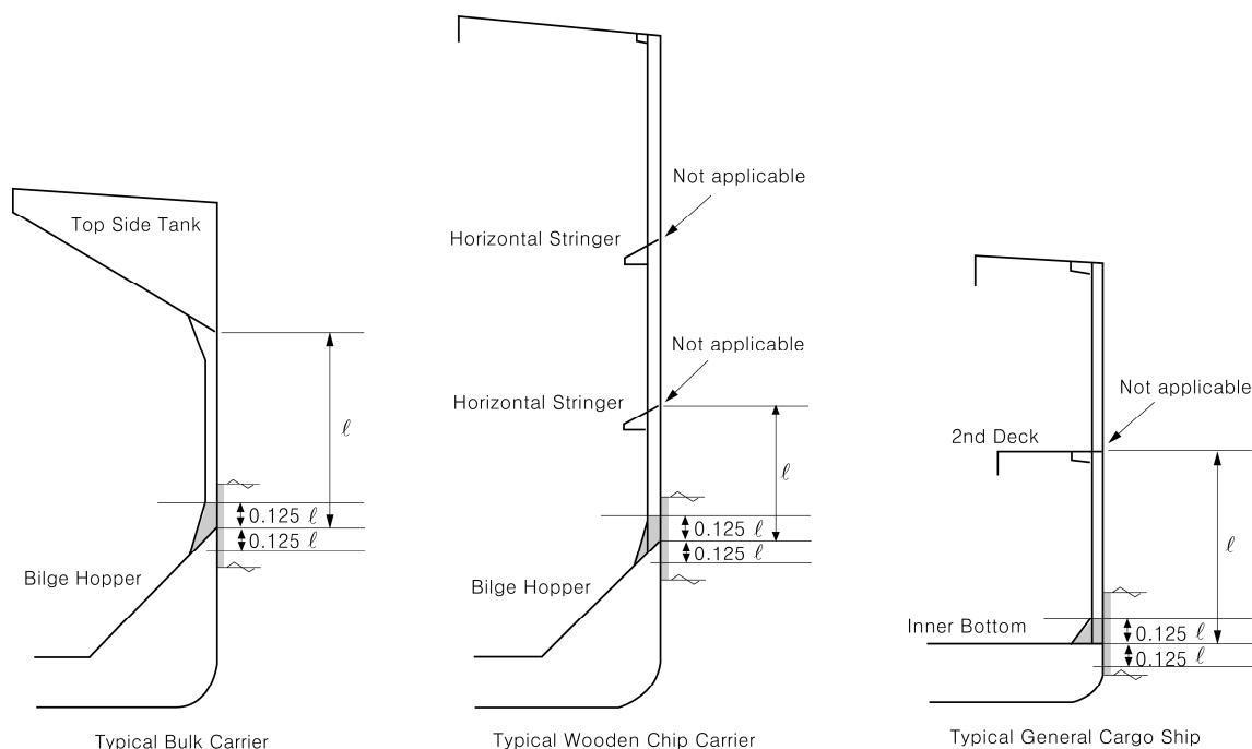
Fig 1 Typical configuration
