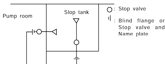
Fig 7.2.21 Examples of piping system of slop tank
