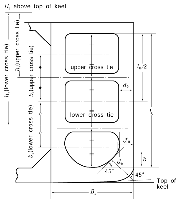
Fig 7.2.2 Measurement of l_0 , d_0 , b and b_s
