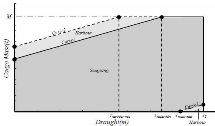
Fig 17 Cargo mass curves
