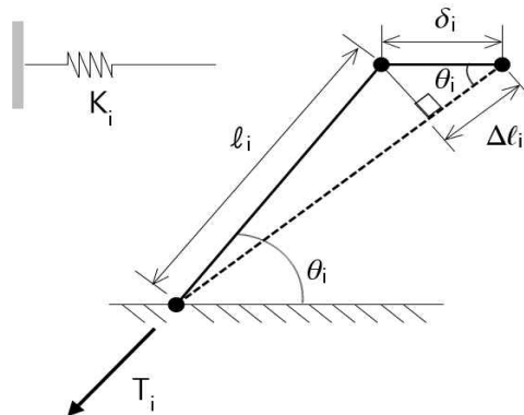
Fig 9 Horizontal stiffness of lashing rod
