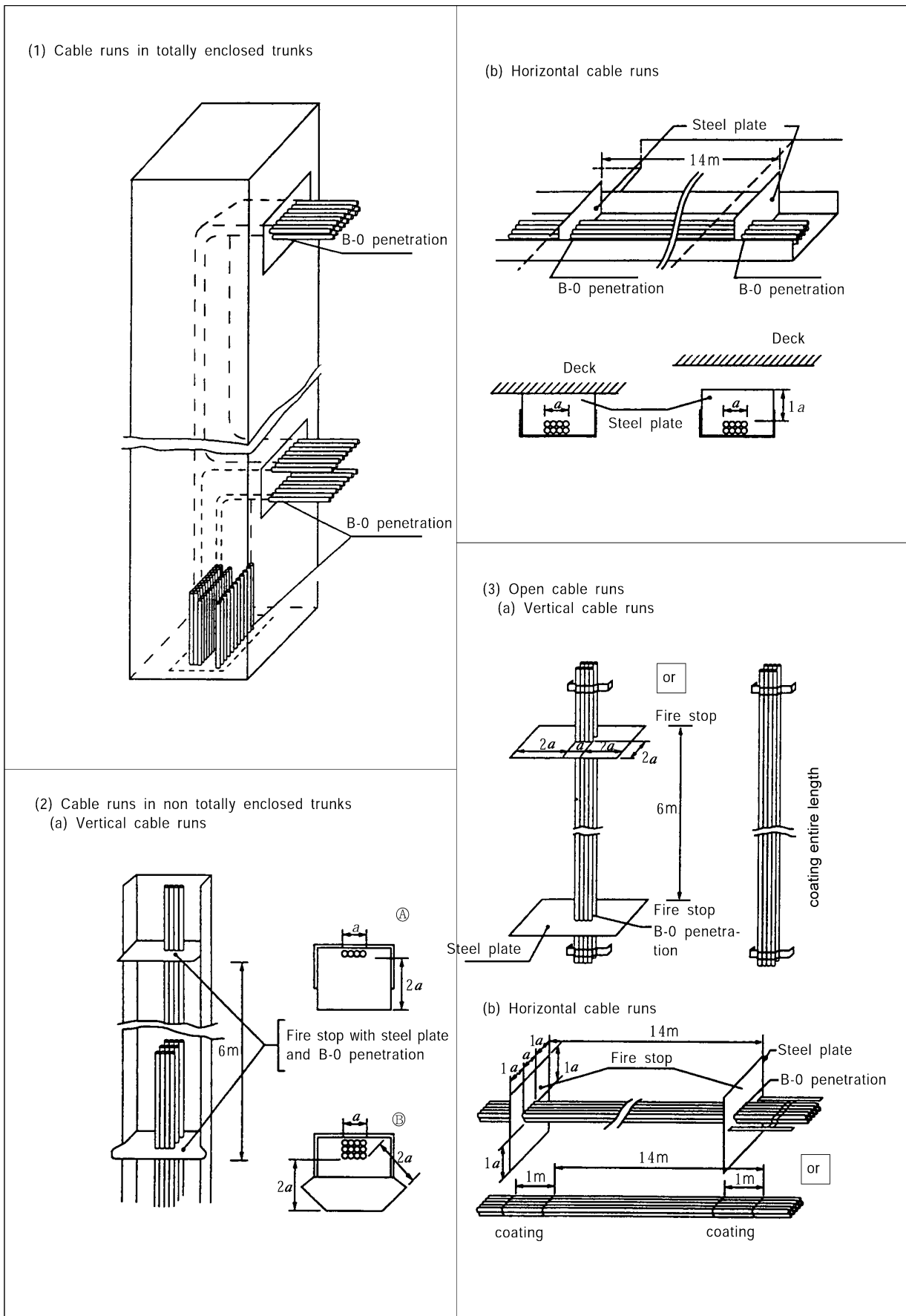
Fig 6.1.5 Flame propagation prevention measures
