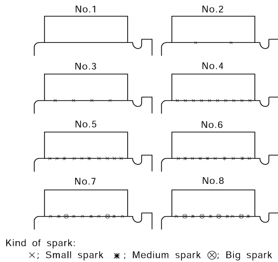
Fig 6.1.4 spark on surface of commutator
