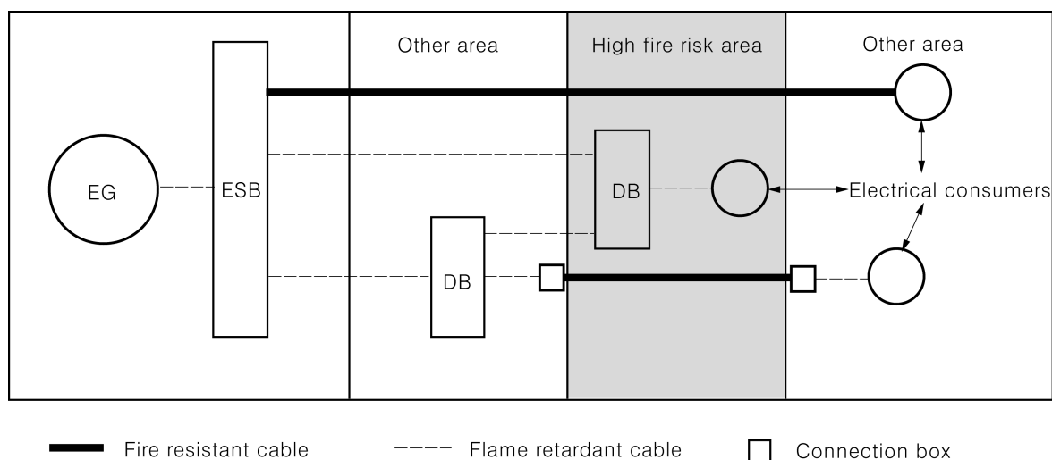
Fig 6.1.6 Example for Application of Fire Resistant Cables
