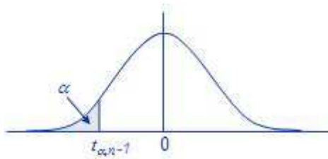
Fig 12 Student's t-distribution
