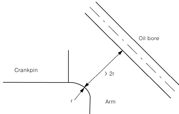
Fig 7 Oil bore proximity to fillet
