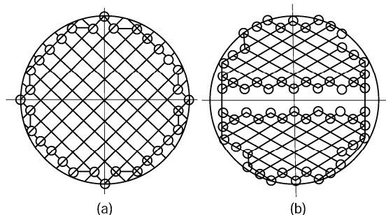
Fig 5.5.4 Polygon Used for Tube Plate Calculation
