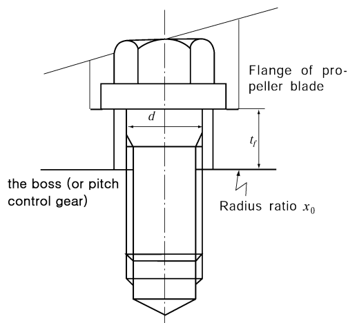
Fig 5.3.3 Measuring Method of Blade Fixing Bolt Dimension
