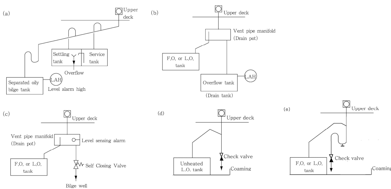
Fig 5.6.3 The Example of Construction Preventing Direct Ingress of Seawater Splashes or Rain Water (2017)
