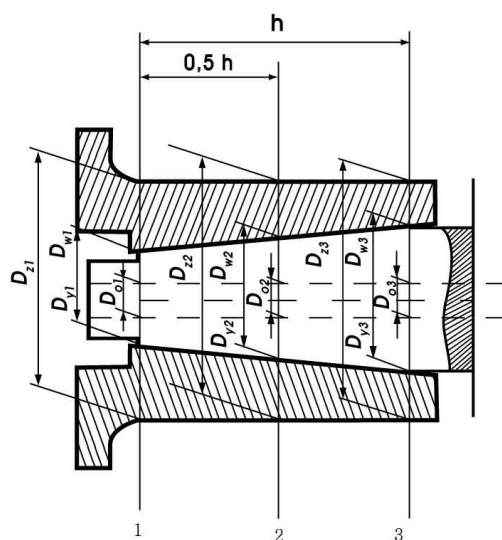
Fig 5.3.1 Details of shaft couplings
