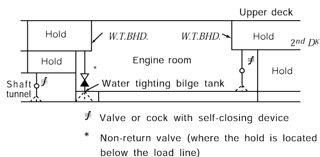
Fig 5.6.8 Example of Hold Bilge Drainage Line through the Watertight Construction
