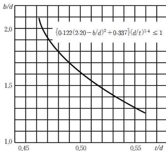
Fig 5.2.1 Relationship between b/d and t/d
