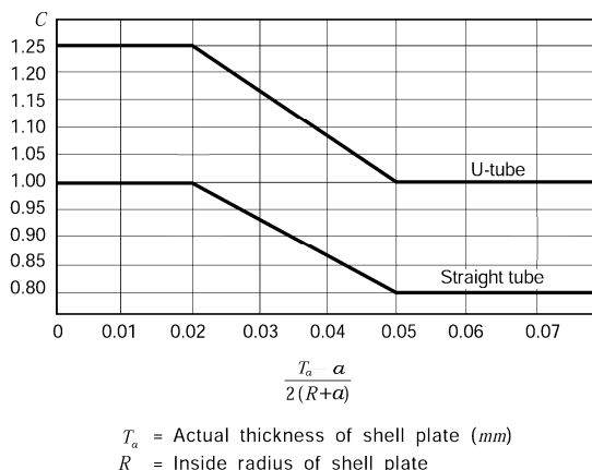
Fig 5.5.3 Value of C
