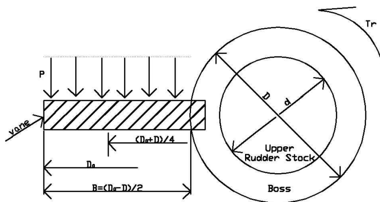
Fig 5.7.2 Rotary vane type rudder actuator
