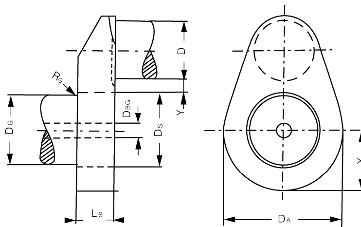
Fig 6 Crankthrow of semi-built crankshaft
