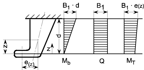
Fig 4.1.6 Rudder horn
