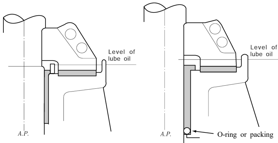
Fig 4.1.14 Rudder carrier
