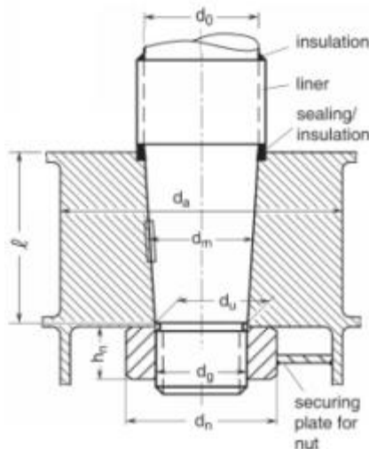
Fig 4.1.6 Cone coupling with key
