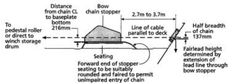
Fig 4.10.2 General arrangement of chain stopper and fairlead
