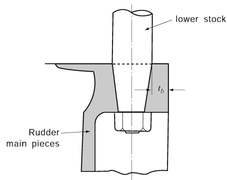
Fig 4.1.12 Coupling between rudder lower stock and rudder main pieces
