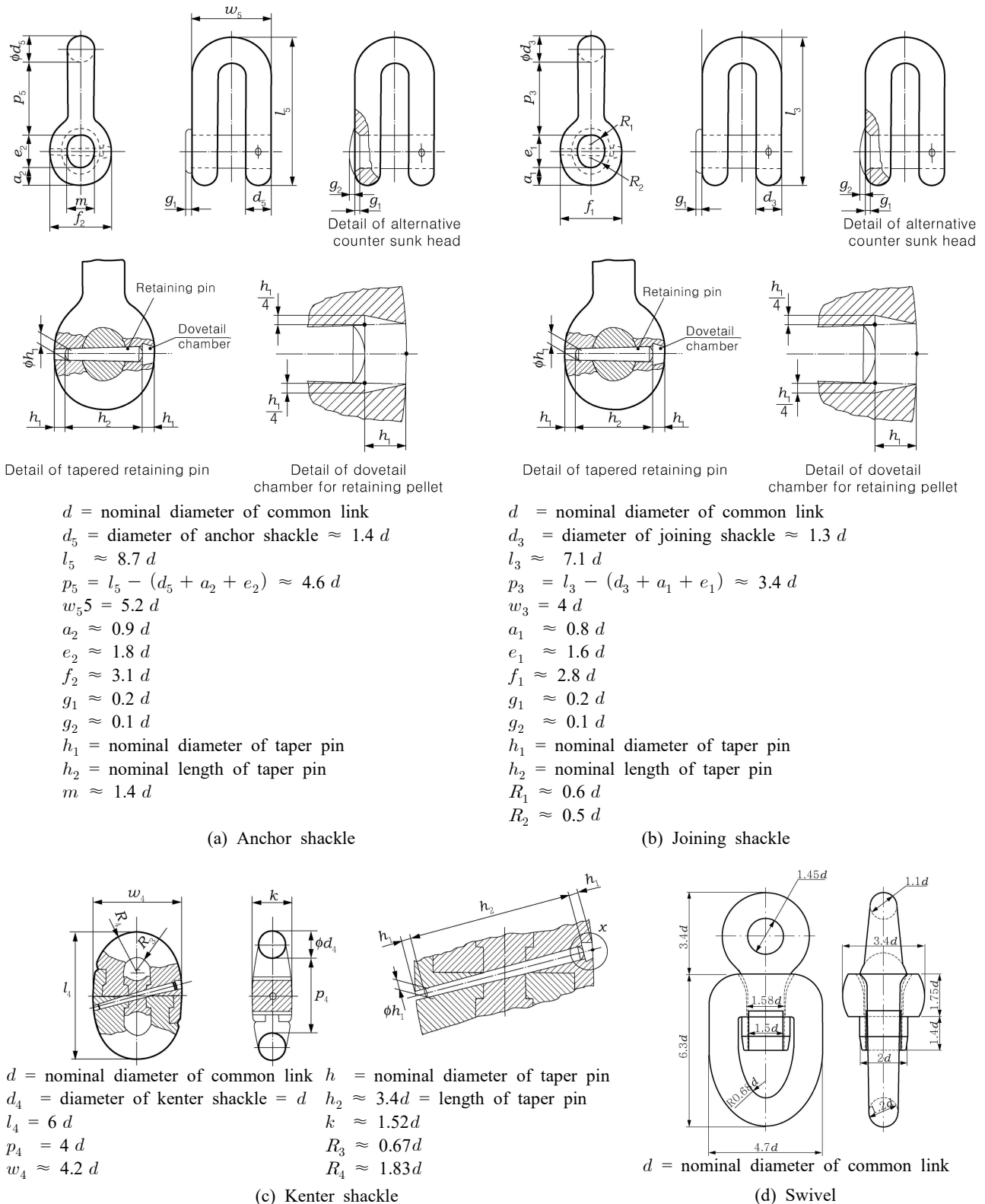
Fig 4.8.4 Shape and proportions of accessories
