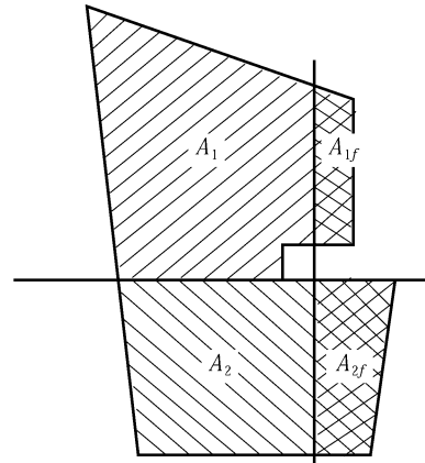
Fig 4.1.3 Division of rudder area
