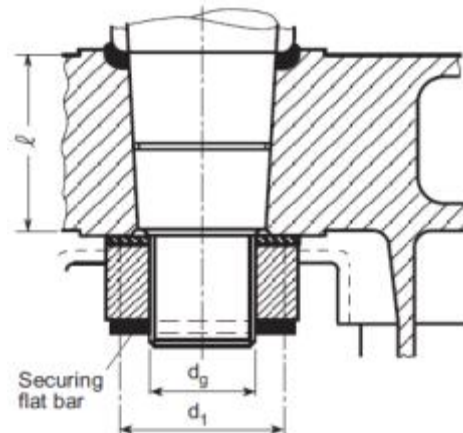
Fig 4.1.7 Cone coupling without key
