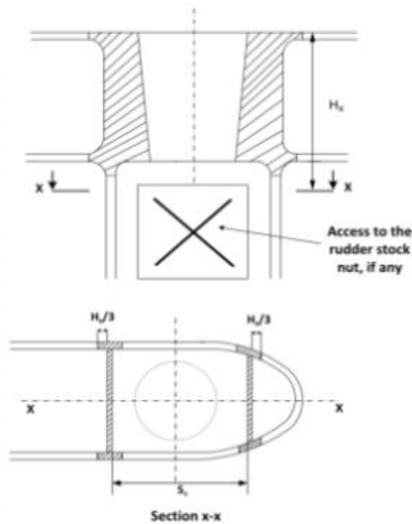
Fig 4.1.4 Connection between rudder structure and rudder stock gudgeon
