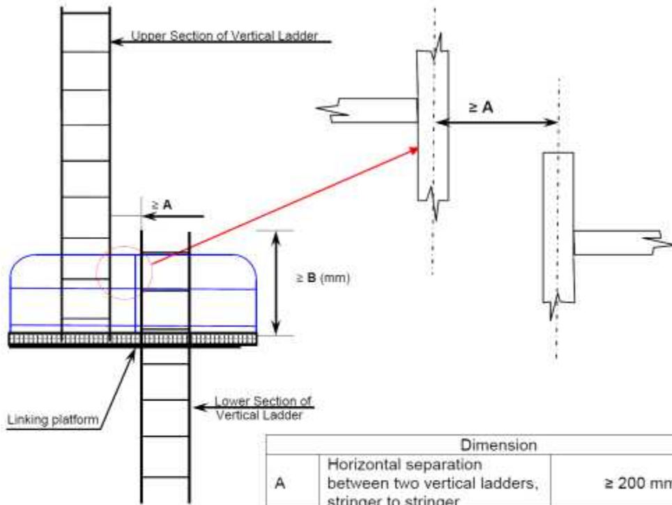
Vertical Ladder - Ladder through the linking platform (2017)
