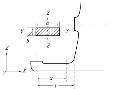
Fig 3.2.1 Shoe piece
