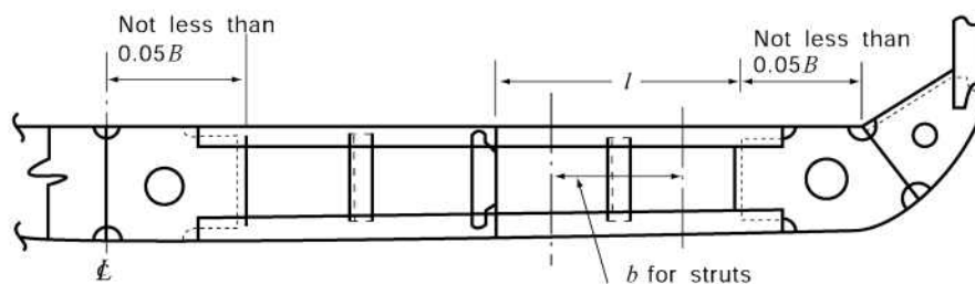
Fig 3.7.1 Open floors
