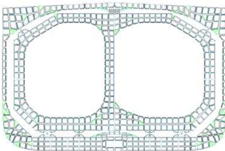
Fig 48 Transverse section
