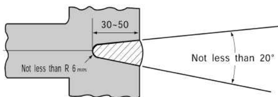
Fig 3.2.1 Welding of cast steel stern frames
