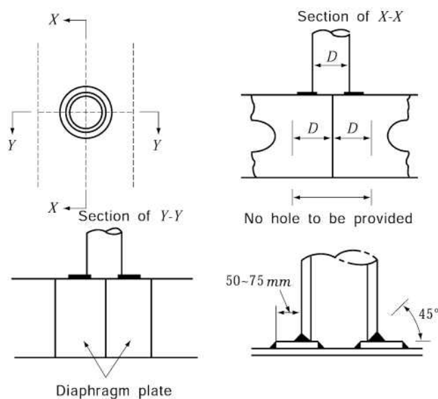
Fig 3.12.1 Compensation of under pillars
