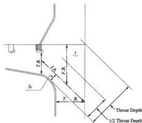
Fig 3.9.4 Compensation of bracket
