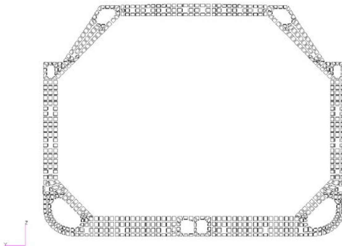
Fig 37 Typical F.E. Model of a transverse web frame
