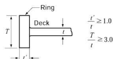
Fig 3.3.4 Reinforcements by ring
