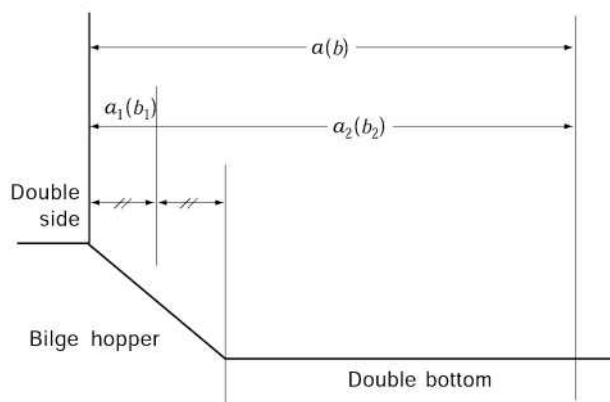
Fig 3.3.6 Measurements of \alpha_1 , \alpha_2 , b_1 and b_2
