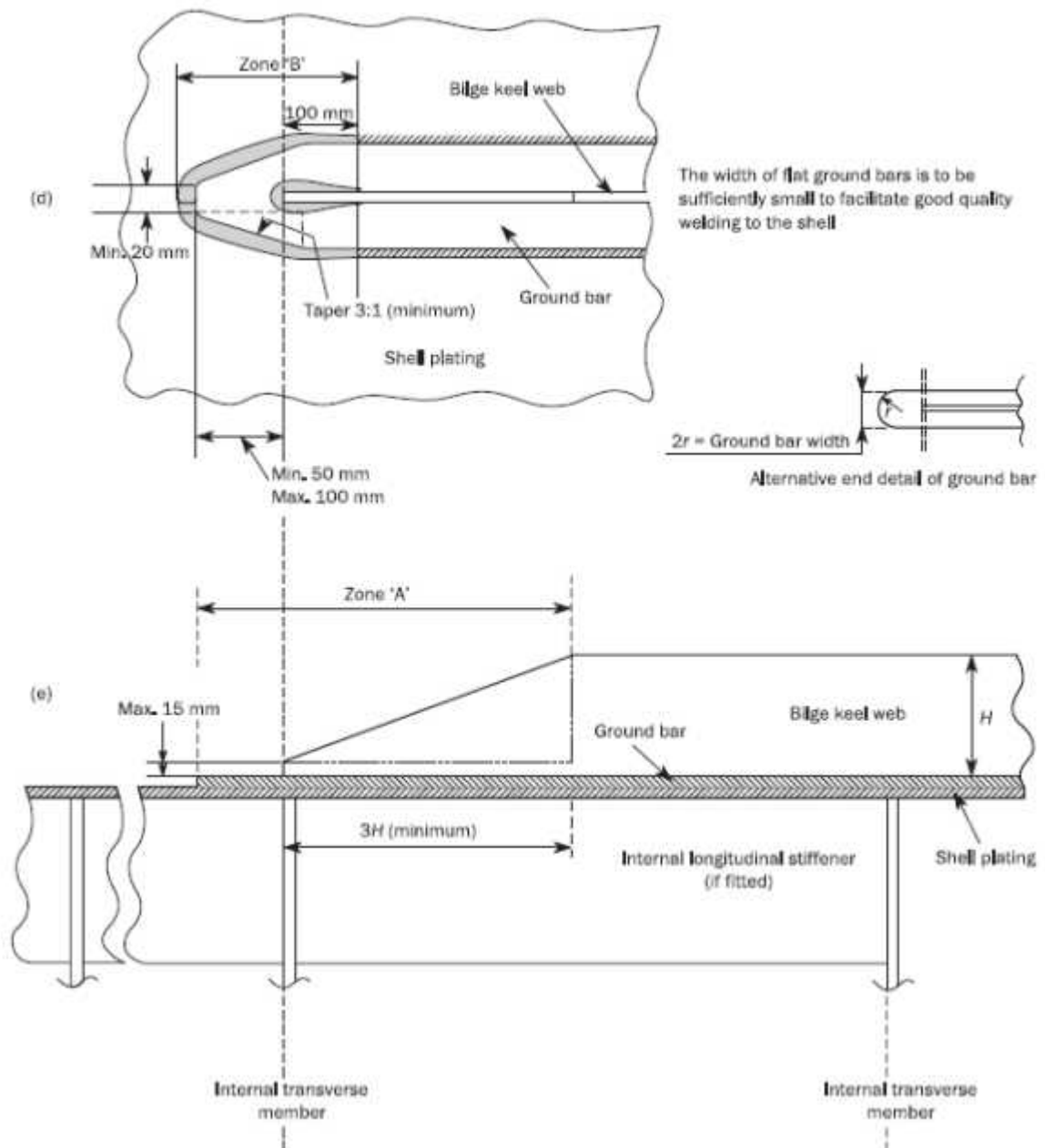
Fig 3.4.3 Bilge keel end design (continued)
