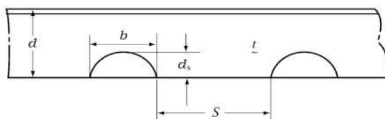
Fig 3.3.1 S , b and d_s of scallops
