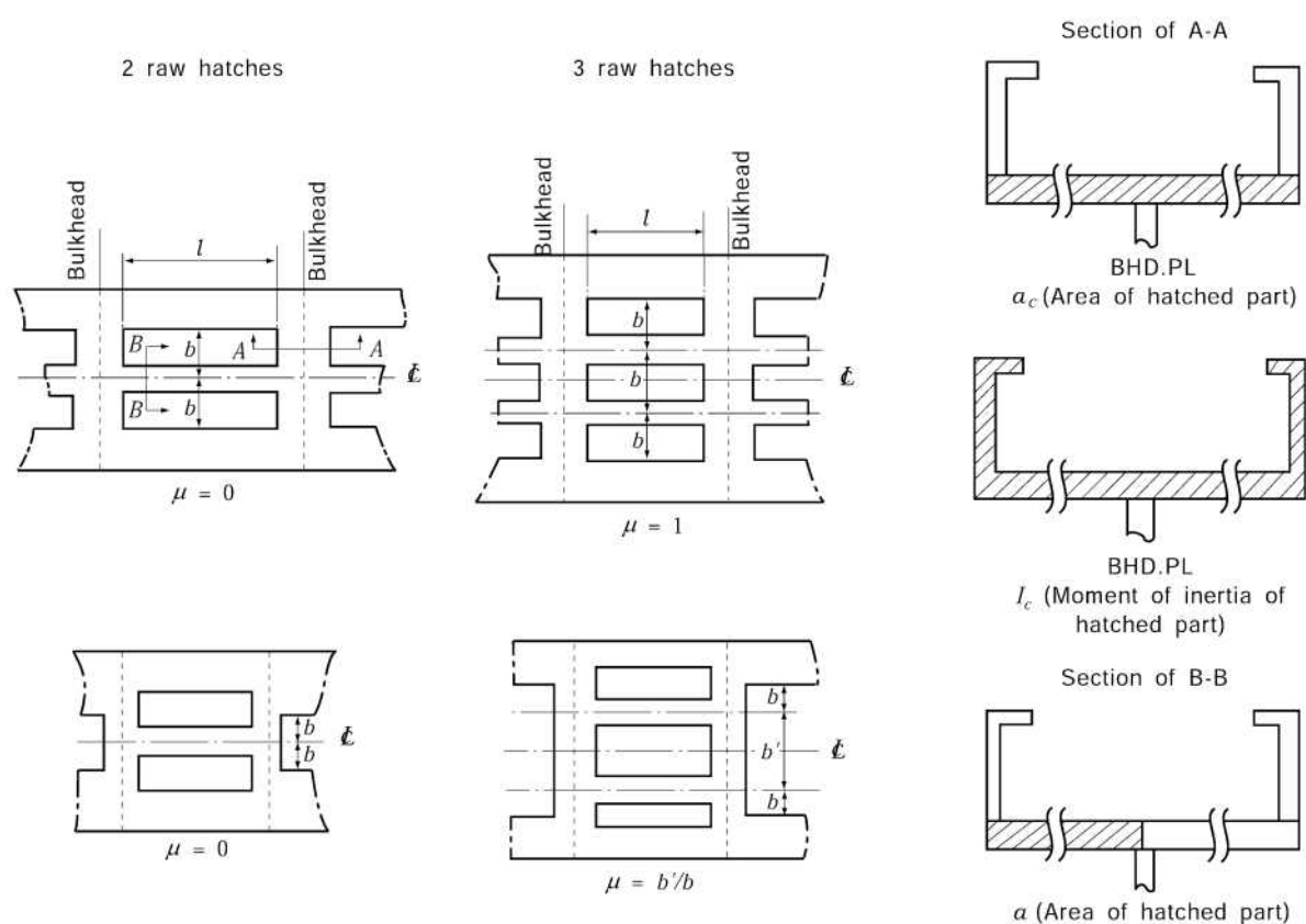
Fig 3.3.2 l , b and \mu
