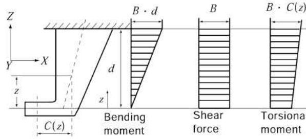
Fig 3.2.2 Rudder horn
