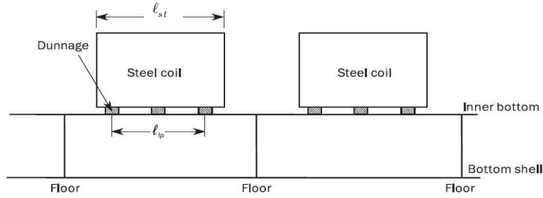
Fig 3 Steel coils loaded between inner bottom floors
