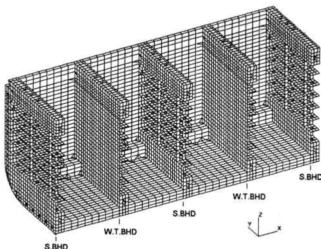
Fig 20 Hold model
