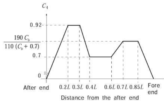
Fig 3.3.6 Value of distribution factor C_4
