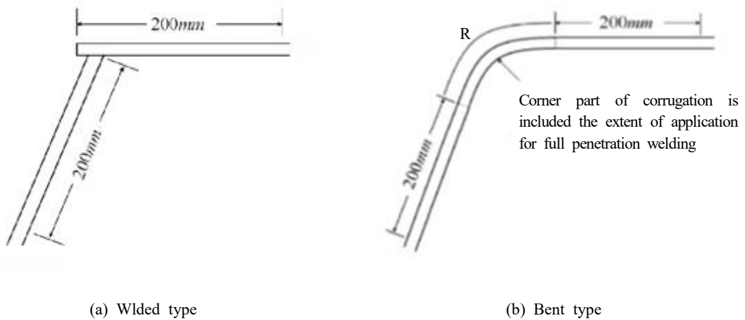
Fig. 3.15.2 Extent of about 200mm from the Corner of the Corrugation
