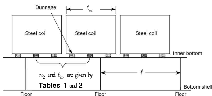
Fig 2 Steel coils loaded independently of inner bottom floors locations
