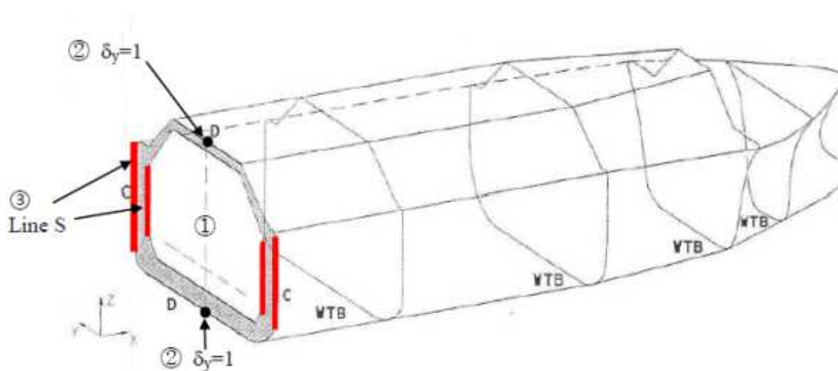
Fig 42 Boundary conditions for vertical dynamic loading condition
