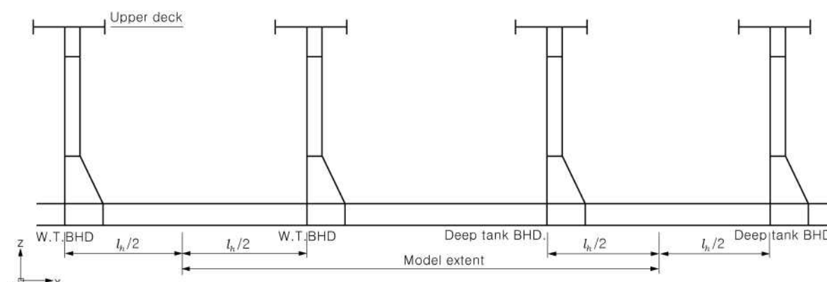
Fig 8 Hold model extent
