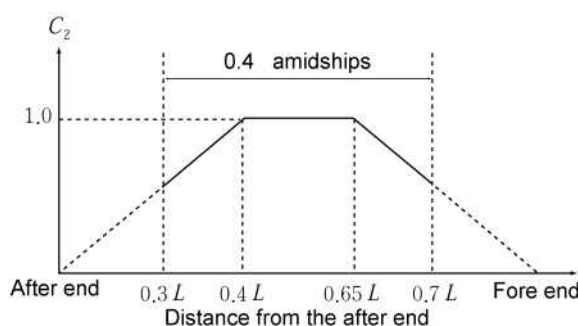
Fig 3.3.2 Value of coefficient C_2
