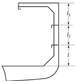
Fig 3.8.4 Transverse hold frames supported by side stringers specially arranged
