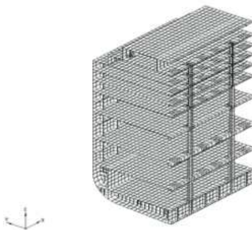
Fig 27 Hold model
