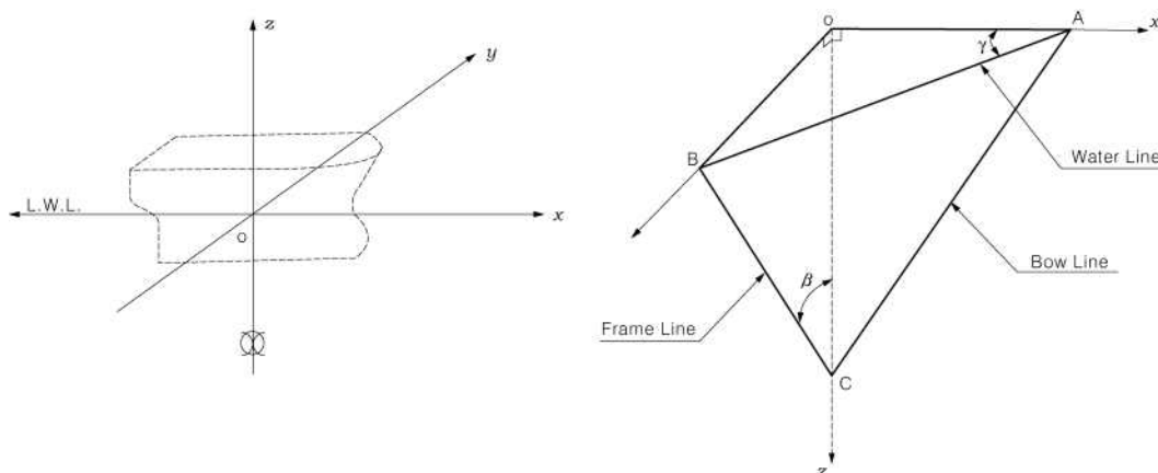
Fig 3.8.3 Shell Angle
