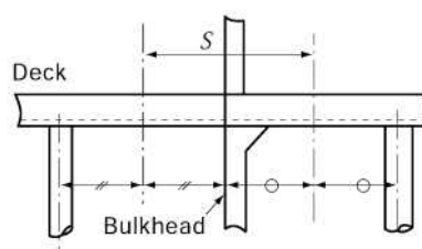
Fig 3.14.2 Measurements of S
