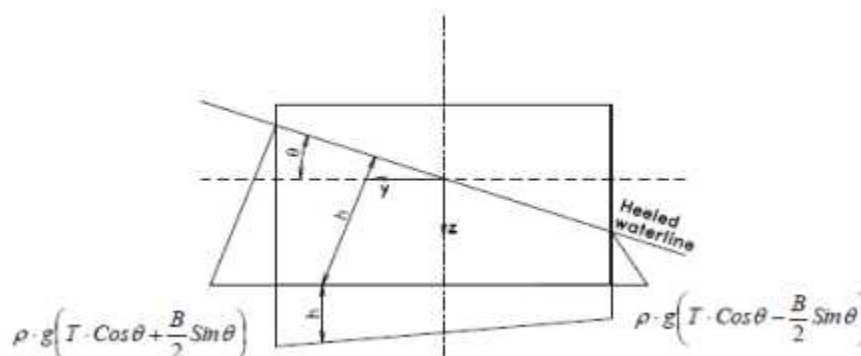
Fig 45 Hydrostatic pressure distribution for transverse heeled
