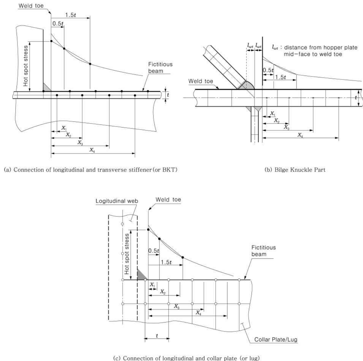
Fig 5 Determination of hot spot stress
