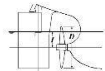
Fig 1 Immersion of propeller
