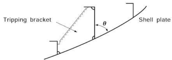
Fig 3.13.1 In case the angle between webs of girders and shell plating is small
