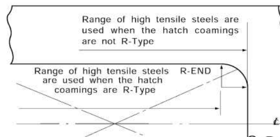
Fig 3.1.8 Hatch coaming
