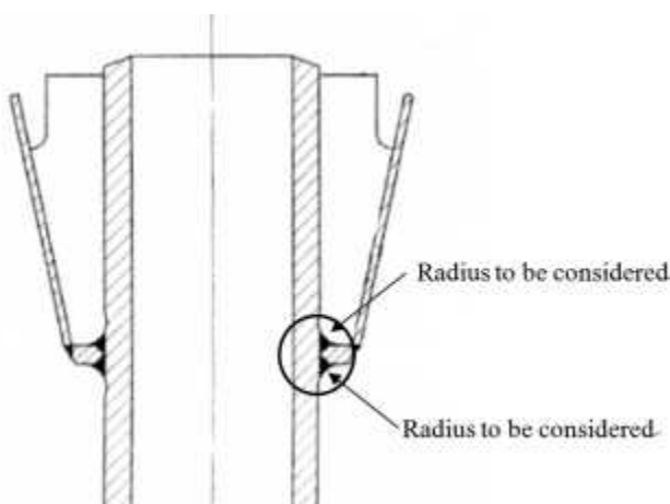
Fig 3.2.7 Fillet shoulder radius
