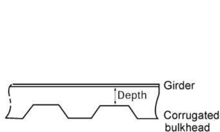
Fig 3.14.7 Measurements of depth of girder
