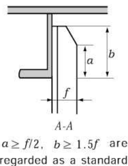
Fig 3.7.8 Details of lap of strut and longitudinal frame
