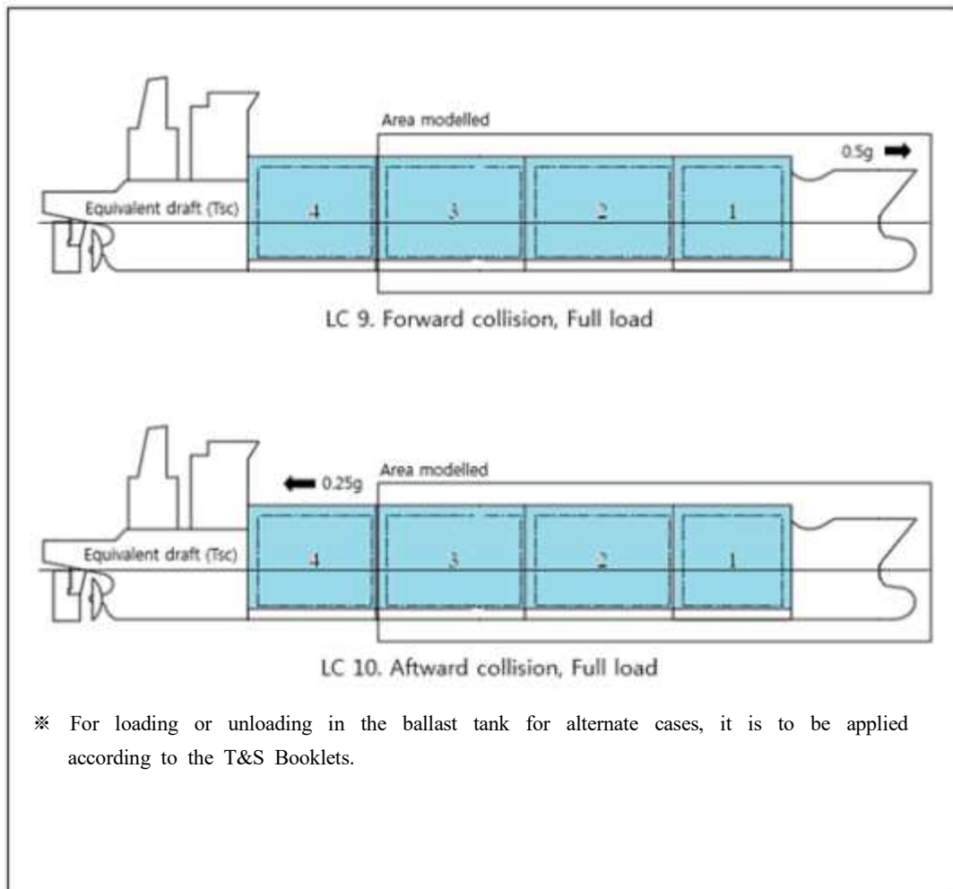
Fig 46 Loading condition(refer to Table 40) (2018)
