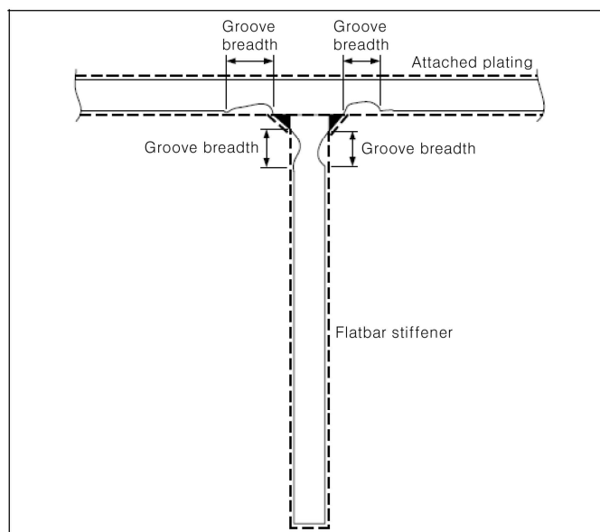
Fig 1.2.3 Grooving corrosion
