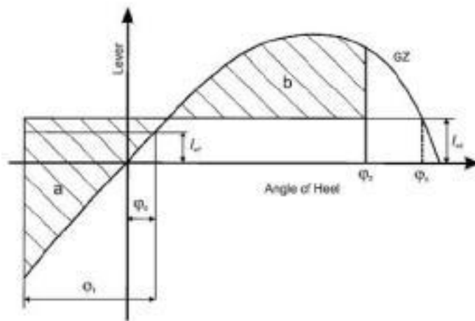
Fig 2.3.1 Severe wind and rolling
