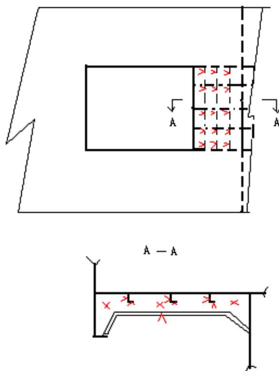
Fig 6 Locations of measurements on underdeck structure
