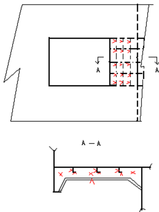
Fig 13 Locations of measurements on underdeck structure
