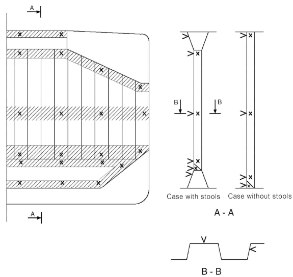
Single skin bulk carriers
