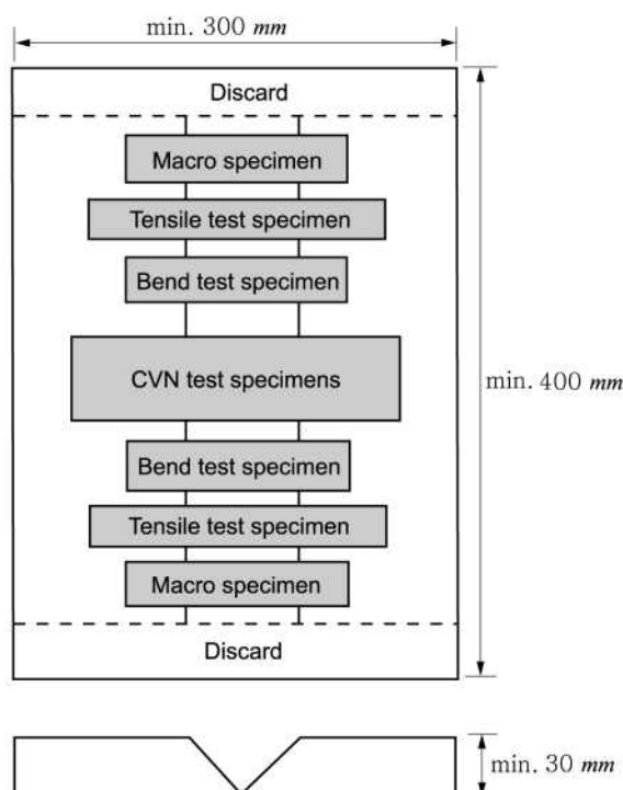
Fig 2.1.6 Test Sample for Butt Welding Test
