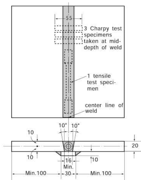
Fig. 2.2.21 Deposited Metal Test Assembly for Electrode for Manual Arc Welding (unit : mm)
