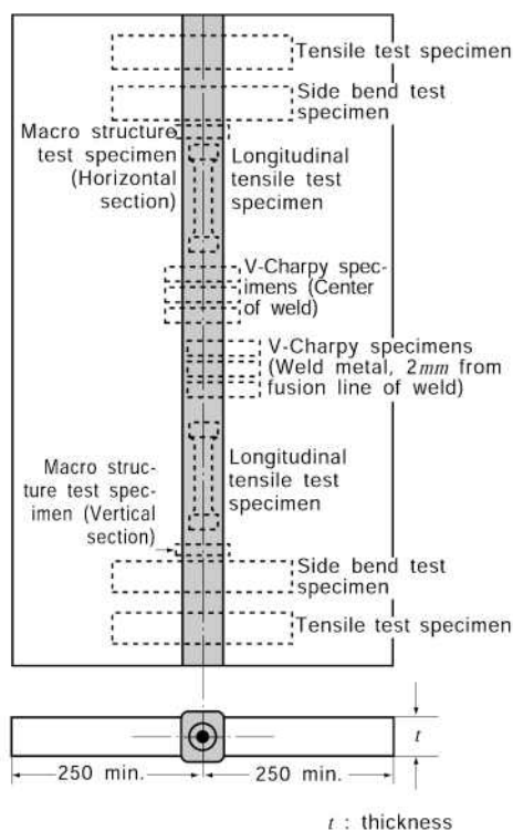
Fig. 2.2.32 Butt Weld Assembly (Electro-slag and electrode-gas welding, Unit : mm)
