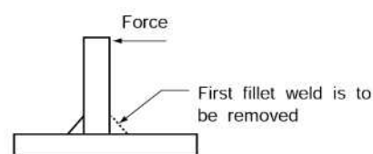
Fig 2.2.6 Hot Cracking Test
