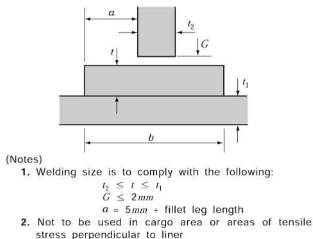
Fig 2.2.3 Fillet Welding inserting a Liner
