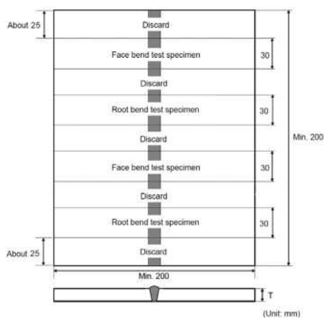
Fig 2.2.12 Dimensions and types of test assembly for butt welds ( T < 12\text{mm} )
