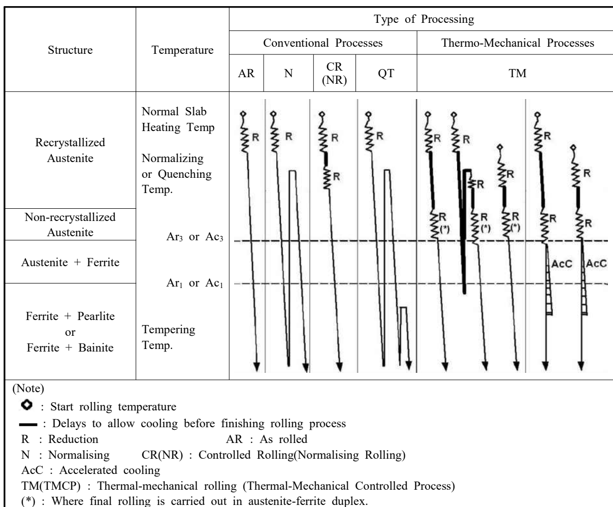
Fig 2.1.5 Rolled Processes for Rolled Steels for Hull
