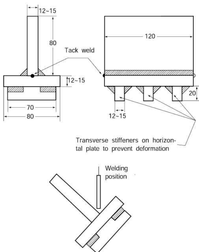
Fig 2.2.5 Hot Cracking Test Assemblies (Units : mm)
