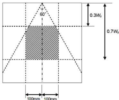
Fig 2.1.4 Necessary conditions of arrest crack position
