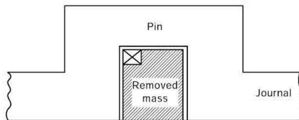
Fig 2.1.7 Location of Test Specimens
