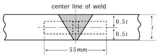
Fig 2.2.22 Position of Butt Weld Impact Test Specimen
