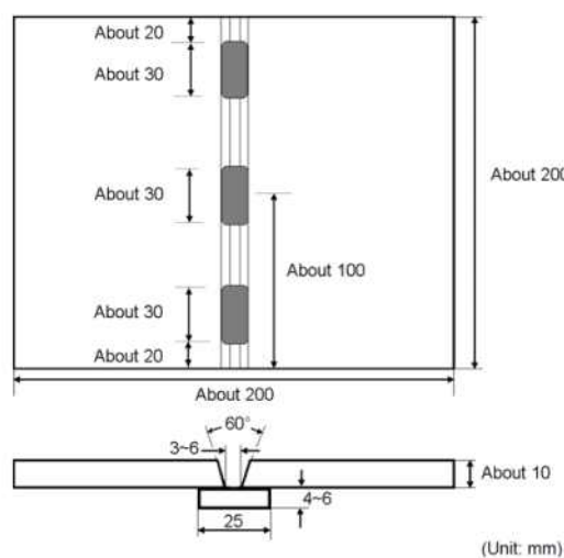
Fig 2.2.15 Dimensions and types of test assembly for tack butt welds
