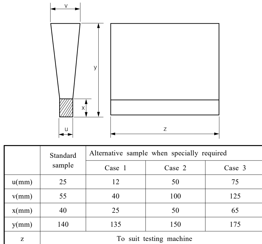
Fig 2.1.16 Y-type test sample
