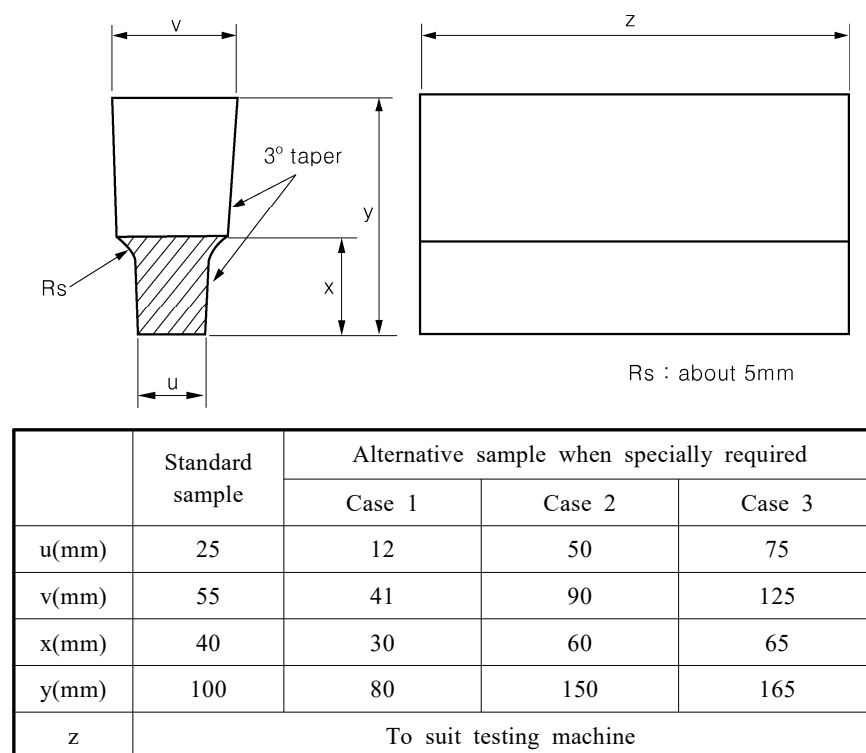
Fig 2.1.14 U-type test sample
