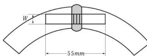
Fig. 2.1.12 The position of selection for impact test specimen taken from the weld zone of electric-resistance welded steel pipes
