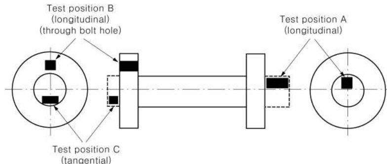
Fig 2.1.18 Flanged shaft
