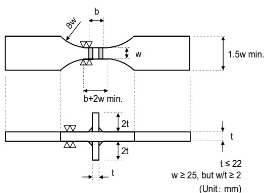
(a) Transverse non-load-carrying fillet welded joint
