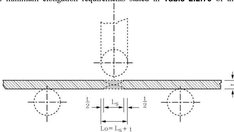
Fig 2.2.42 gauge length L 0
