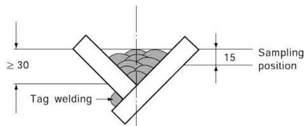
Fig. 2.2.39 Deposited Weld Metal Test Assembly (Unit : mm)
