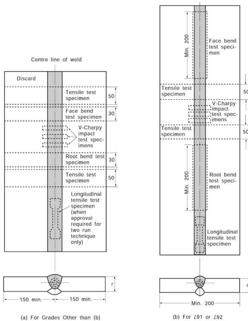
Fig. 2.2.29 Butt Weld Test Assembly with Two-run Technique (Automatic welding, Unit : mm, t : plate thickness)
