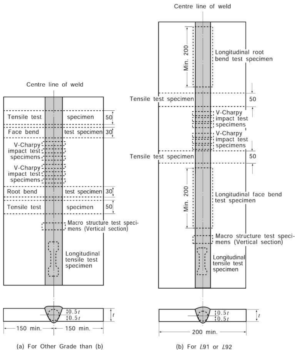
Fig. 2.2.34 Butt Weld Test Assembly with One-run and Multi-run Technique (Unit : mm, t= Plate thickness)
