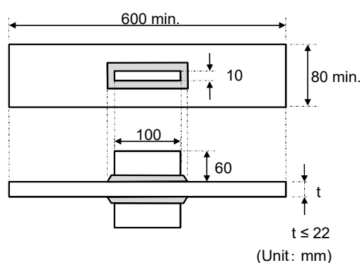
(b) Longitudinal fillet welded gusset
