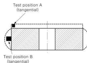
Fig 2.1.21 Gear wheel
