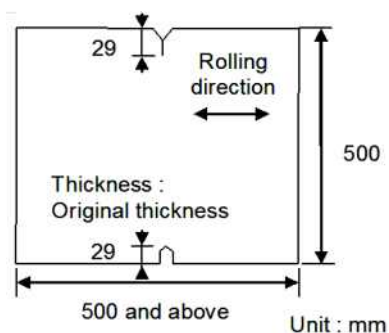
Fig 2.1.3 Shape and size of specimen
