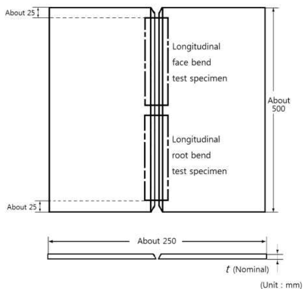
Fig 2.2.14 Dimensions and types of test assembly for butt welds (For 9%nickel alloys)
