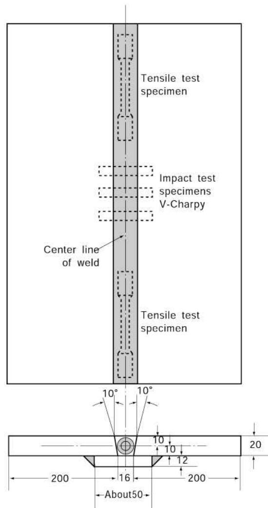
Fig. 2.2.27 Deposited Metal Test Assembly with Multi-run Technique (Automatic Welding, Unit : mm)
