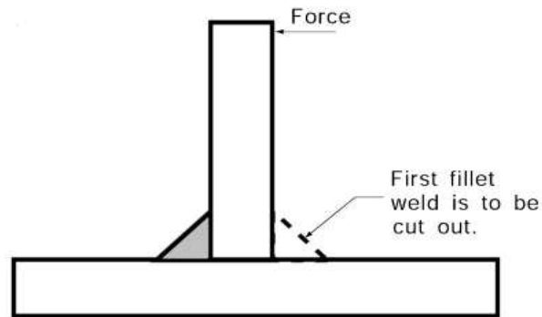
Fig 2.2.26 Fracture Test
