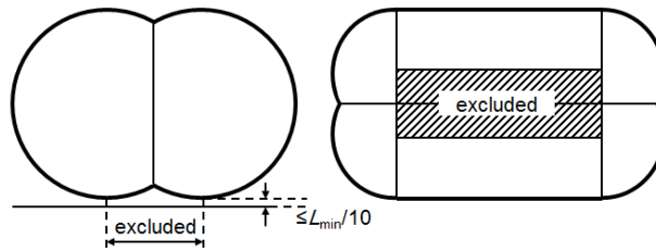
Bilobe tank
