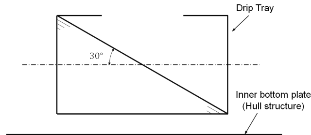
Fig. 6.1 Drip Tray to protect the inner bottom plate
