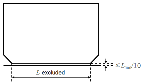
Prismatic tanks
