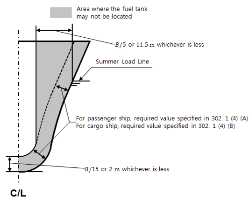
Fig 5.1 Location of Fuel Tank
