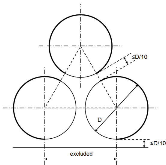
Horizontal cylindrical tanks arrangement
