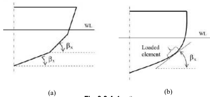
Fig 3.2.4-1 \beta_X
