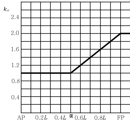
Fig 3.2.1 Longitudinal Distribution Factor for Vertical Design Acceleration k_v
