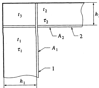
Fig 3.3.6 Bracketless Joint
