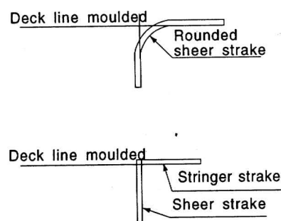
Fig 3.3.3 Deck Corners
