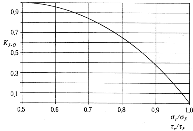
Fig 3.1 Factor K_{J-O}
