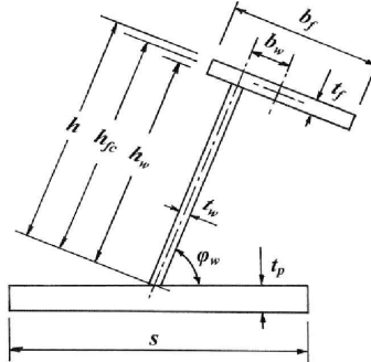
Fig 2.4 Stiffener geometry
