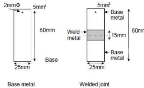
Fig 3.32.5 Test piece
