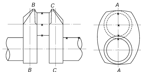
Fig 2.5.1 Sampling Positions
