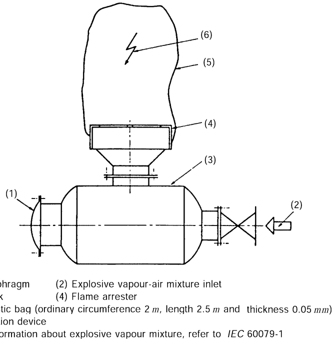
Fig 3.24.2 Example of Testing Equipment for Flame Arrester
