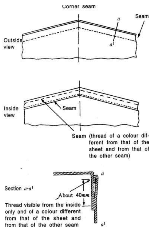
Fig 3.1 Sheets Made of Several Pieces
