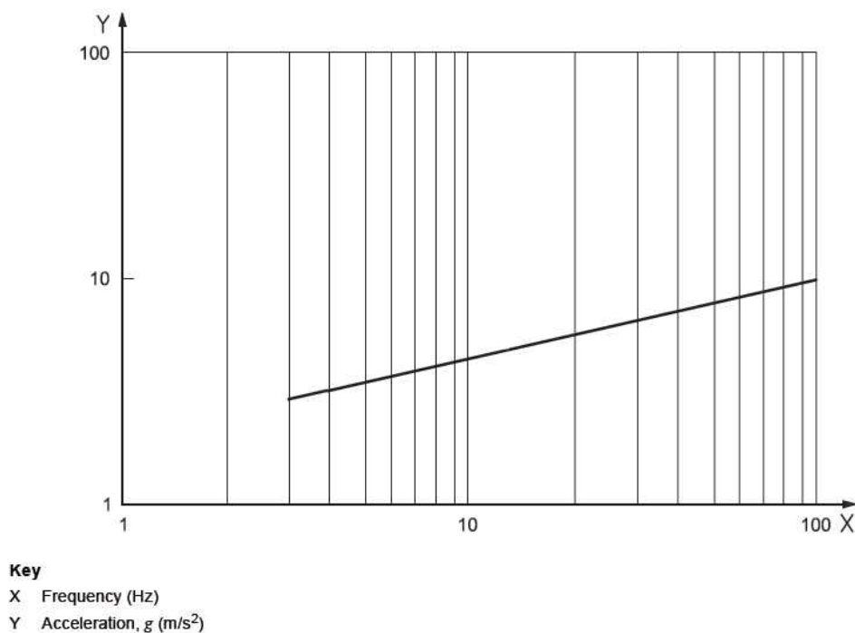
Fig 2.28 Minimum SRS Curve (5 % Damping)
