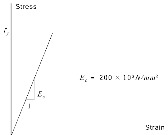
Fig. 3.6.2 Stress-Strain Relation for Non-Prestressed Steel in Uniaxial Tension
