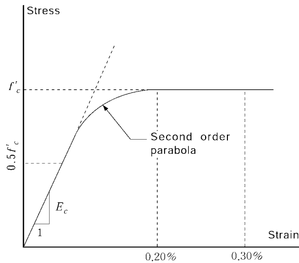
Fig 3.6.1 Stress-Strain Relation for Concrete in Uniaxial Compression
